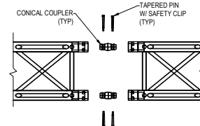
TRUSS TO TRUSS CONNECTION 1-1/2" = 1'-0"
